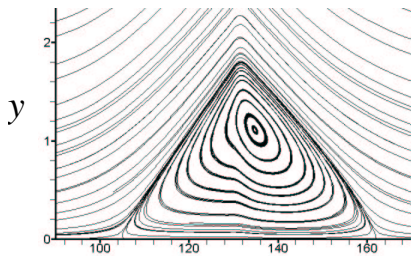
Figure 15: Enlarged view of the separation bubble
