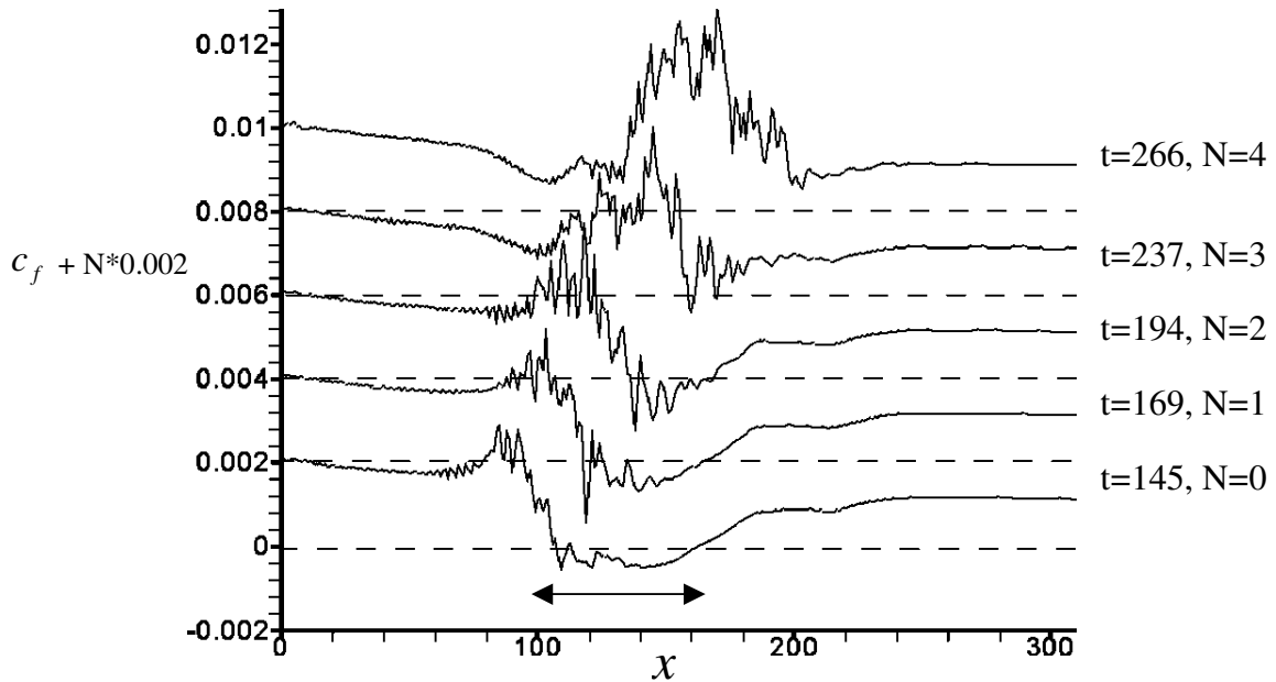
Figure 24: Skin friction distribution. The arrowed region (shows the bubble interaction zone for 100 < x < 165 )
