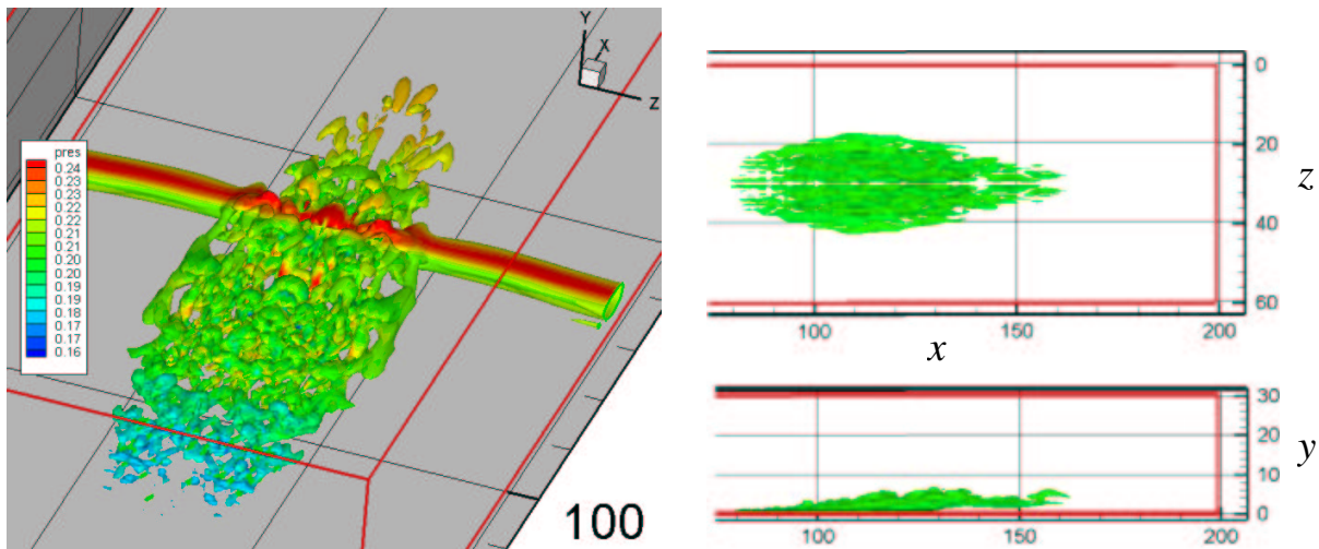
Figure 17: Spot sub-structures ( \Pi = -0.003 ) superimposed with the static pressure values ( t = 169 )
